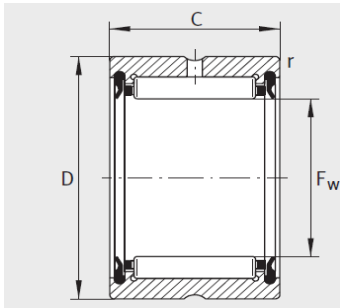
RNA4903-2RSR
